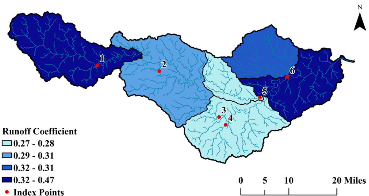
Figure 4.1. Index Points and runoff coefficient analysis for the Upper Iowa River Watershed. This figure shows the runoff coefficients for the simulation period (2002-2016).
