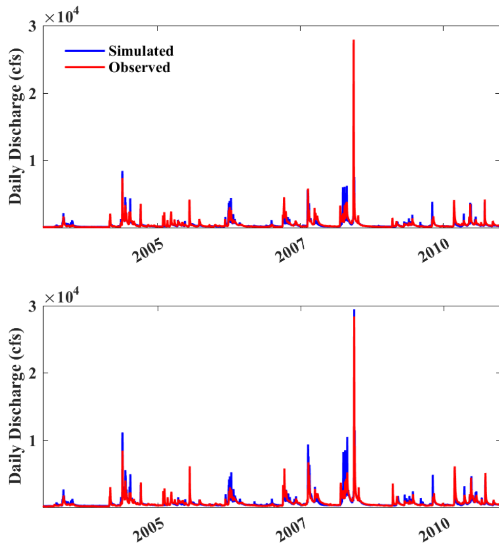
Figure 3.4. Observed and simulated daily flow time series. Calibration period. Top: Decorah (USGS 05387500) and bottom: Dorchester (USGS 05388250).
