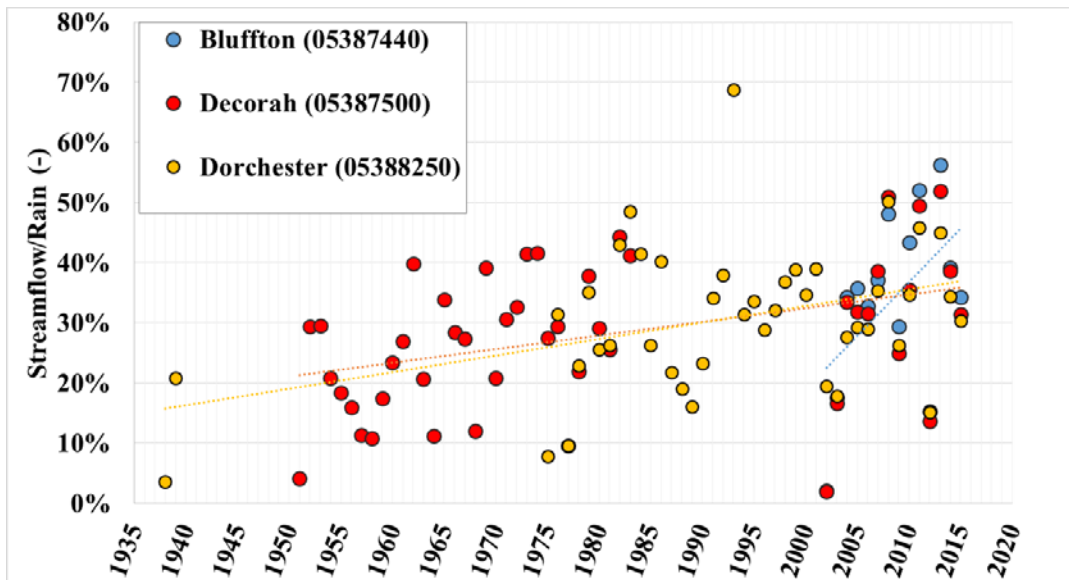
Figure 2.4. Annual ratio of streamflow to precipitation.
