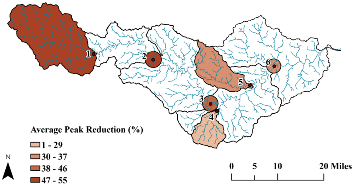
Figure 4.4. Average peak discharge reduction (%) for index points in the Upper Iowa River Watershed. Baseline vs. Native Vegetation (historic precipitation).
