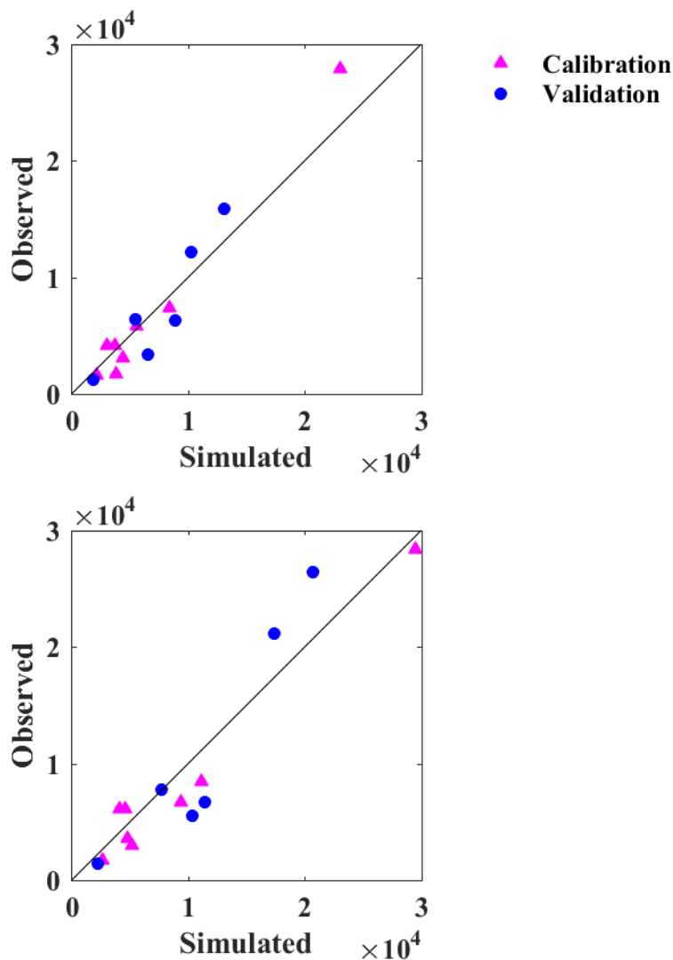
Figure 3.7. Simulated versus observed annual maximum peak daily discharges (cfs). Top: Decorah (USGS 05387500) and bottom: Dorchester (USGS 05388250).
