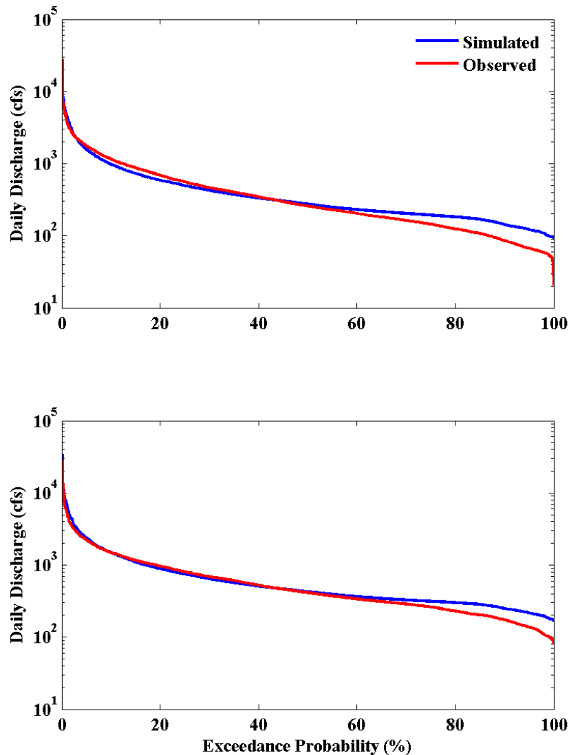
Figure 3.8. Daily flow duration curves. Top: Decorah (USGS 05387500) and bottom: Dorchester (USGS 05388250).
